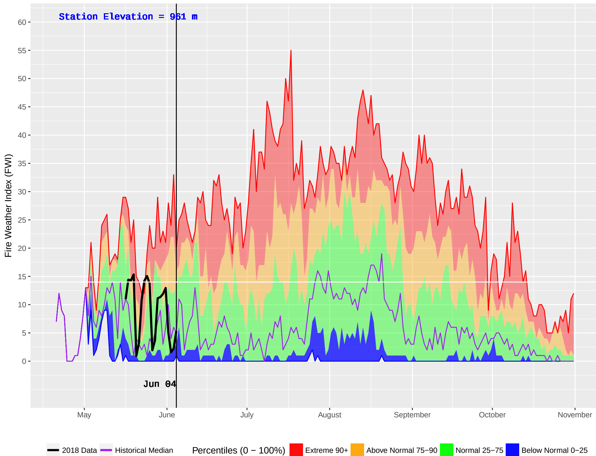
HOLY CROSS 2 (654) : Historical (1998–2016) and Current (2018) Noon Fire Weather Index (FWI)
