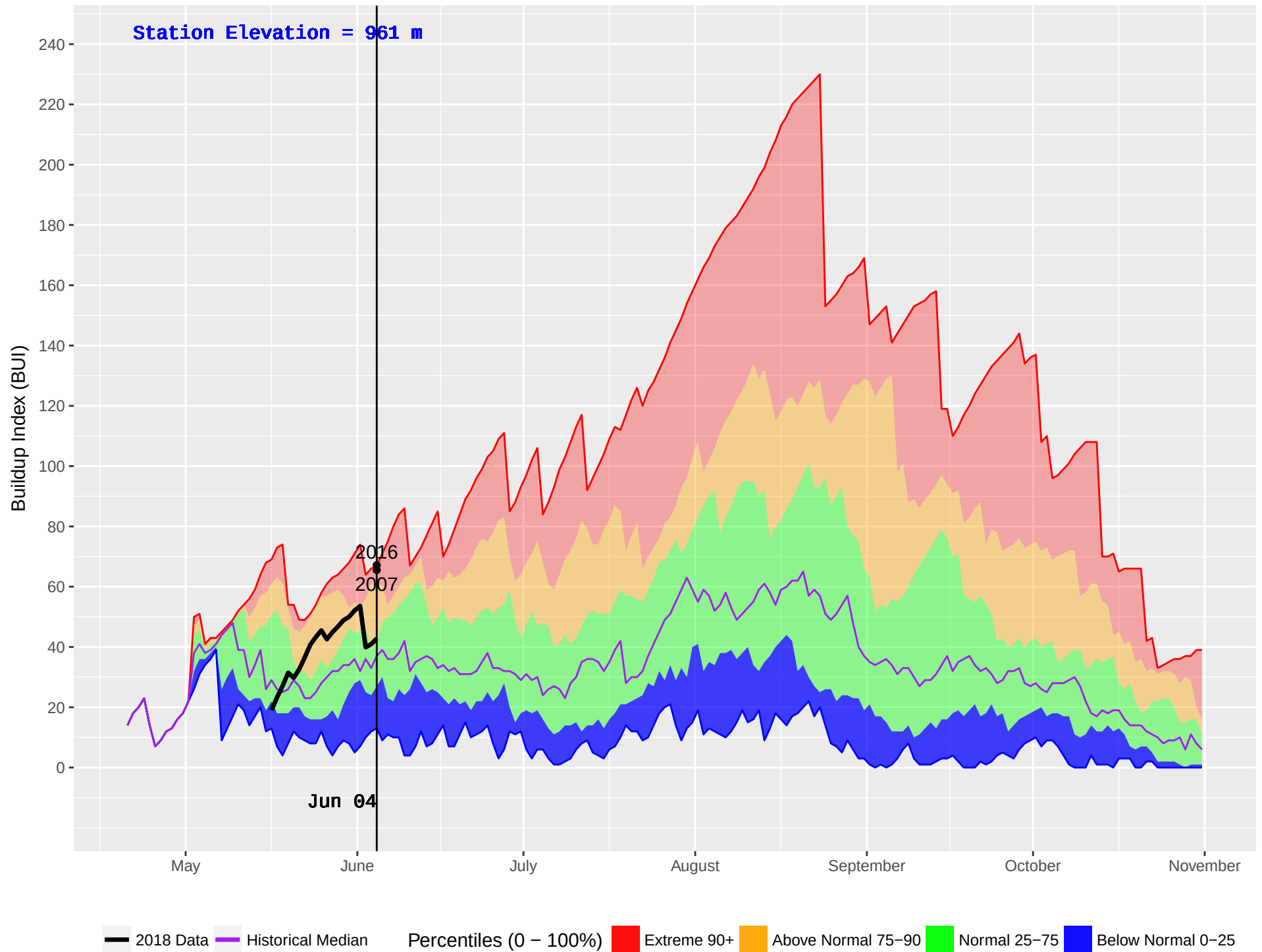
HOLY CROSS 2 (654) : Historical (1998–2016) and Current (2018) Noon Buildup Index (BUI)
