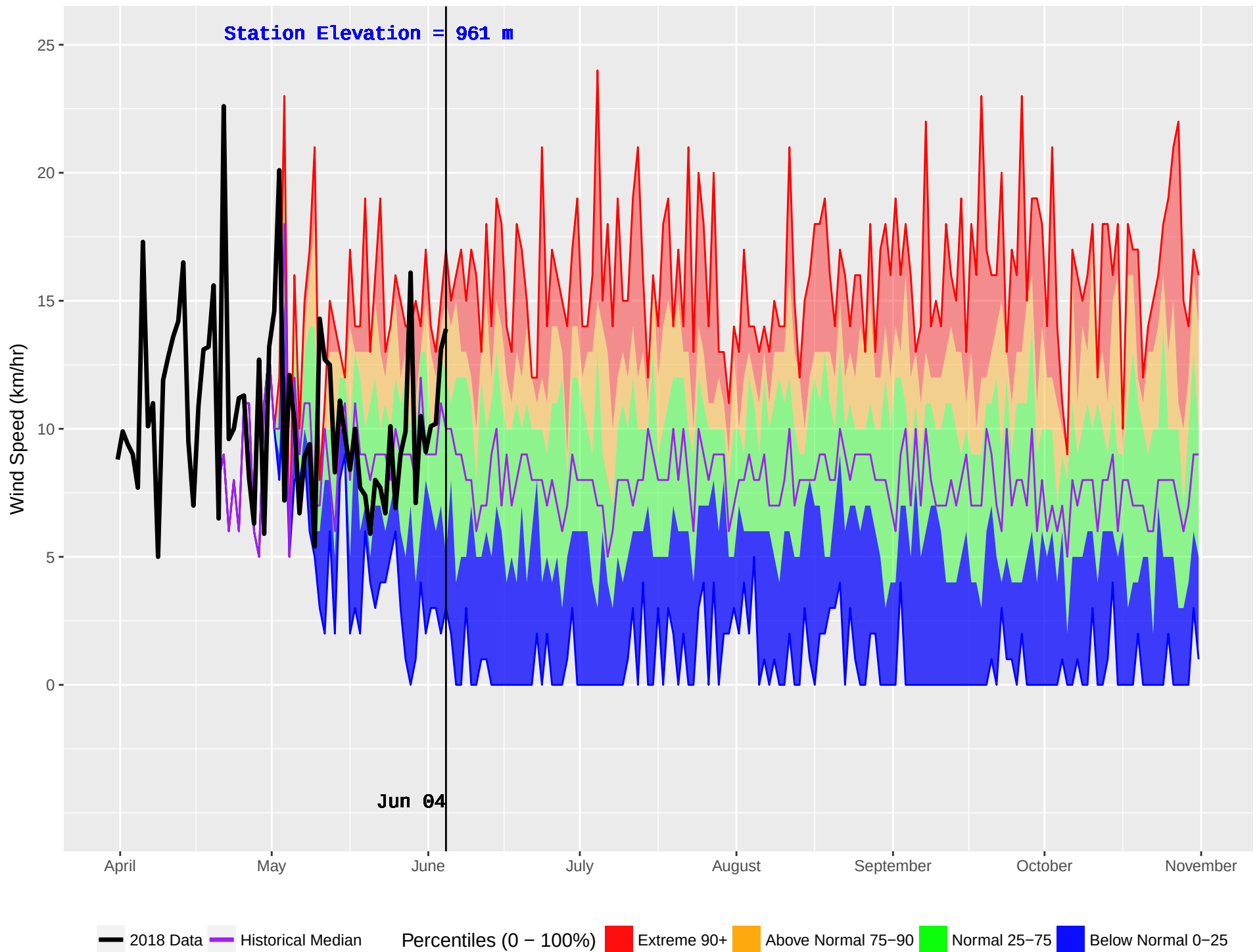
HOLY CROSS 2 (654) : Historical (1998–2016) and Current (2018) Noon Wind Speed
